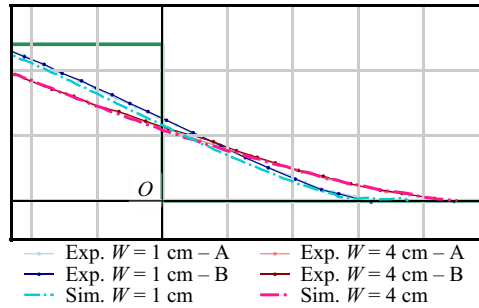
Figure 14. Influence of the sidewalls: rest-state height profiles of simulated and experimental collapses for a = 1 and two different widths ( W = 1 \text{ cm} and W = 4 \text{ cm} ) at 0^\circ slope. Two experimental replicates (A and B) are compared for each width run. The green solid line delineates the initial column with size 0.12 \times 0.12 \text{ cm}^2 . Numerical collapses are performed with a constant internal friction coefficient \mu = 0.44 and a friction coefficient between the glass walls and the material \mu_w = 0.23 .
