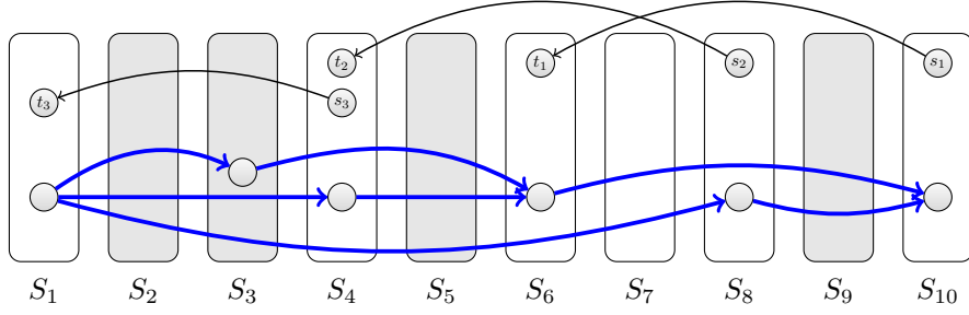
Figure 3: A nice decomposition of a strong semicomplete digraph with three backwards arcs (in thin black). The grey sets (S_2, S_3, S_5, S_9) are ignored. The thick blue arcs are regular-bad.
