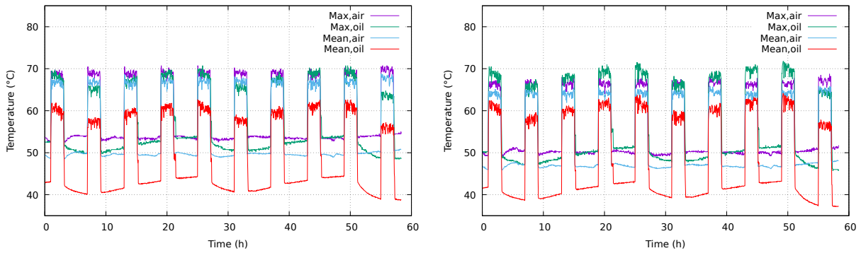
Fig. 3. Average temperature of the mean and maximal cores temperatures for the CPU0 (left) and CPU1 (right) during the LU tests.
