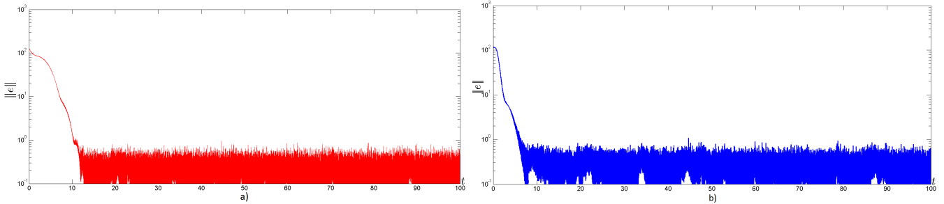
FIGURE 2 Simulation plot of \|e\| for the finite-time a) and fixed-time b) observers with measurement band limited noise of power 10^{-5} and initial conditions x(0) = 10^2(0, 1, \pi/4, 0)^T
