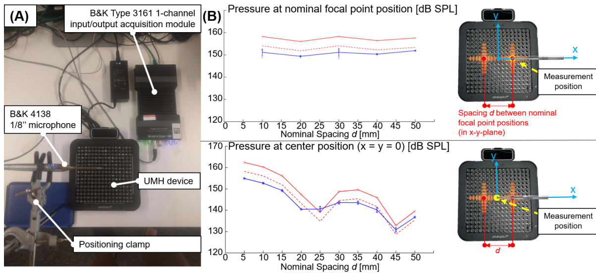
Fig. 6. (A) Microphone recording setup for validation measurements. (B) Plots showing the measured (blue) vs. simulated (red) pressure at the focal point nominal positions for 5 spacing values (top), as well as the mean pressure at the center position between both nominal positions ( x=0,y=0 in the array coordinate system) (bottom). Circles indicate data points while lines show the mean and error bars show one standard deviation. The dashed red line shows the pressure expected for AM focal point pairs based on the simulation of unmodulated focal point pairs, i.e. with a -4.2 dB offset applied.
