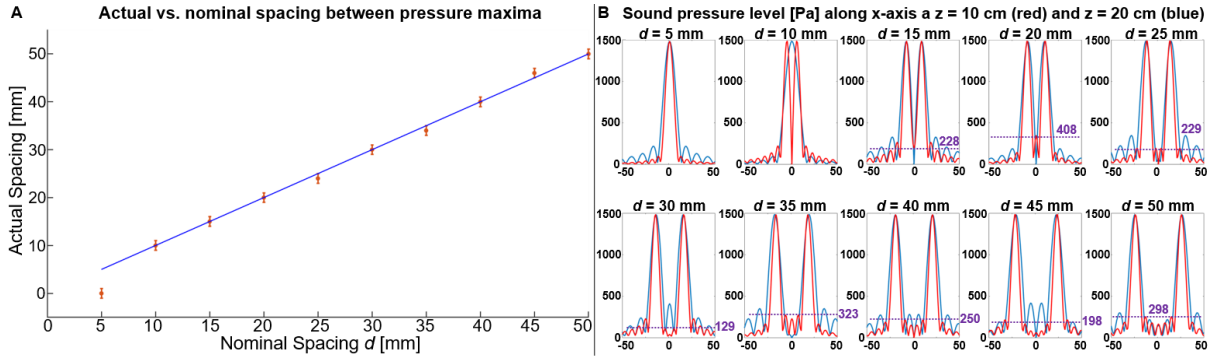
Fig. 9. Simulation of focal point pairs with identical spacing to those used in the human participant study, on the same array, but at a height of z=10 cm above the array. (A) shows the relationship between actual and nominal spacing. (B) shows plots of the acoustic pressure along the x axis in red, overlaid on the plots from Fig. 7 (at z=20 cm) in blue.
