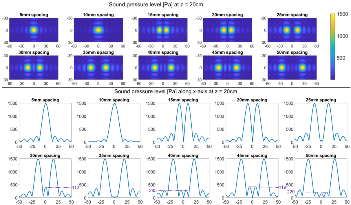
Fig. 7. (Top) Heat maps showing the sound pressure level in the plane at z=20\text{cm} above the array (in Pa). (Bottom) Sound pressure plots along the y=0 axis in the same plane (in Pa). Notable pressure lobes occurring between the peaks around the focal points are annotated with their peak pressure value (in Pa) in purple.
