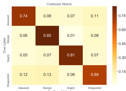
Figure 5: Proposed method
