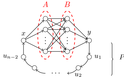
■ Figure 2 A directed graph where the shortest Eulerian walk has length \Omega(|V||E|) = \Omega(|V|^3) .
