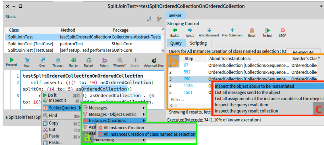
Figure 1: SeekerOC interface. To the left, the Time-Travelling Queries menu(a) available in the code presenter. To the right, the Query Results Table(b) and its context menu(c).
