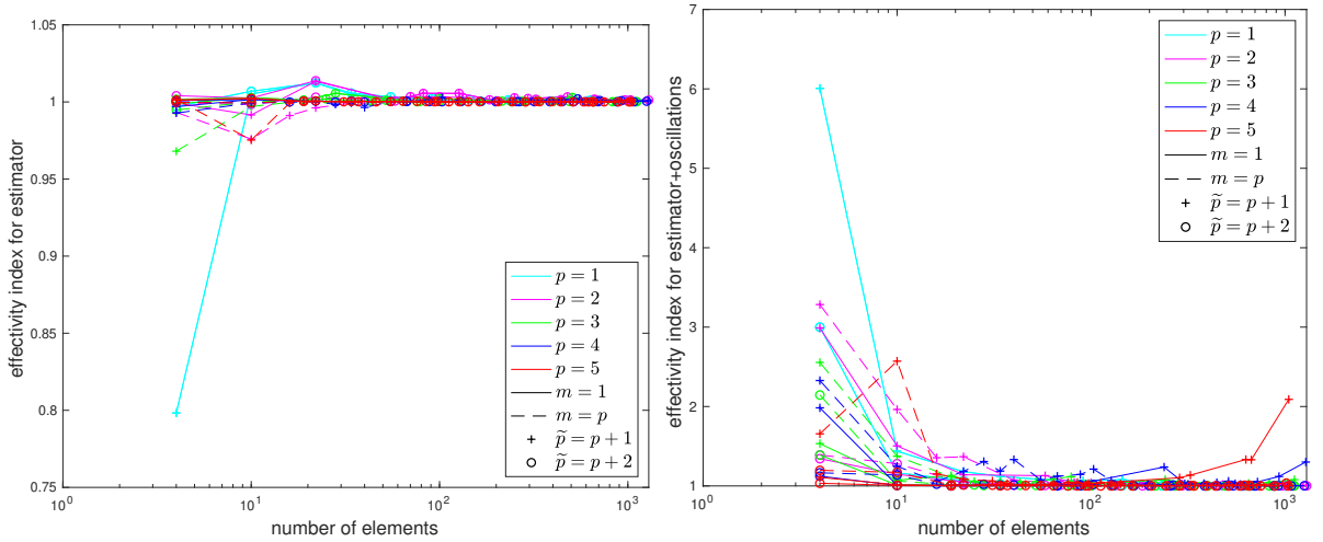
FIGURE 9. Effectivity indices \frac{\|\sigma_h + \nabla u_h\|_\Omega}{\|\nabla(u - u_h)\|_\Omega} (left) and \frac{\|\sigma_h + \nabla u_h\|_\Omega + \text{osc}_h^{\text{rel}}}{\|\nabla(u - u_h)\|_\Omega} (right) corresponding to the problem of Section 9 with adaptive mesh refinement, polynomial degrees p \in \{1, \dots, 5\} , multiplicities m \in \{1, p\} .
