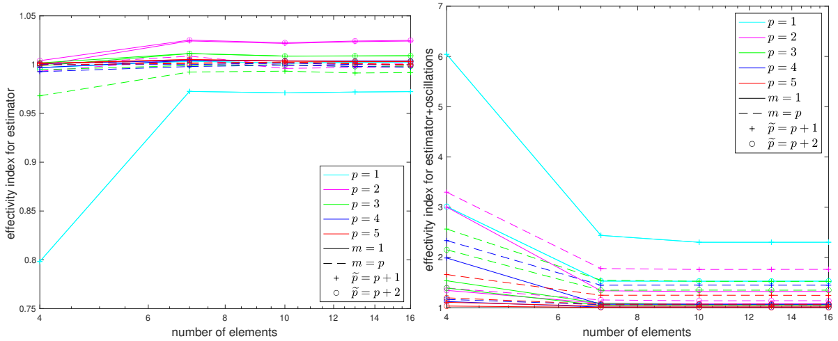
FIGURE 11. Effectivity indices \frac{\|\sigma_h + \nabla u_h\|_{\Omega}}{\|\nabla(u - u_h)\|_{\Omega}} (left) and \frac{\|\sigma_h + \nabla u_h\|_{\Omega} + \text{osc}_h^{\text{rel}}}{\|\nabla(u - u_h)\|_{\Omega}} (right) corresponding to the problem of Section 9 with artificial refinement enforcing a high number of overlapping patches (see Figure 7, bottom), polynomial degrees p \in \{1, \dots, 5\} , multiplicities m \in \{1, p\} .
