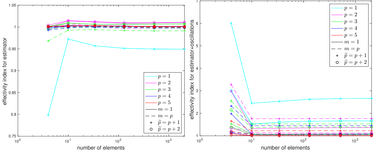
FIGURE 10. Effectivity indices \frac{\|\sigma_h + \nabla u_h\|_\Omega}{\|\nabla(u - u_h)\|_\Omega} (left) and \frac{\|\sigma_h + \nabla u_h\|_\Omega + \text{osc}_h^{\text{rel}}}{\|\nabla(u - u_h)\|_\Omega} (right) corresponding to the problem of Section 9 with artificial refinement enforcing a high number of hanging nodes (see Figure 7, top), polynomial degrees p \in \{1, \dots, 5\} , multiplicities m \in \{1, p\} .
