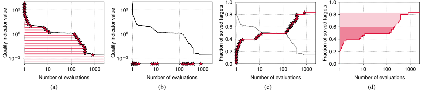
Fig. 2. Construction of the (anytime) empirical runtime distribution (RTD) from the quality indicator convergence graph and equally spaced target values. The lengths of the horizontal lines in (a) represent the runtime measurements for different target values taken from the quality indicator convergence graph, as do the stars in (a)–(c). When the target values are evenly spaced on the given y -axis, the RTD reconstructs, up to discretization, the lower envelope of the convergence graph flipped upside down, (c). The areas above the RTD in (d) represent average runtimes, in that the logarithm of the geometric average of a fraction of the smallest runtimes equals the area size divided by the trim fraction. The dark area corresponds to the shortest 60%, dark plus light area correspond to the fraction of all solved problems.
