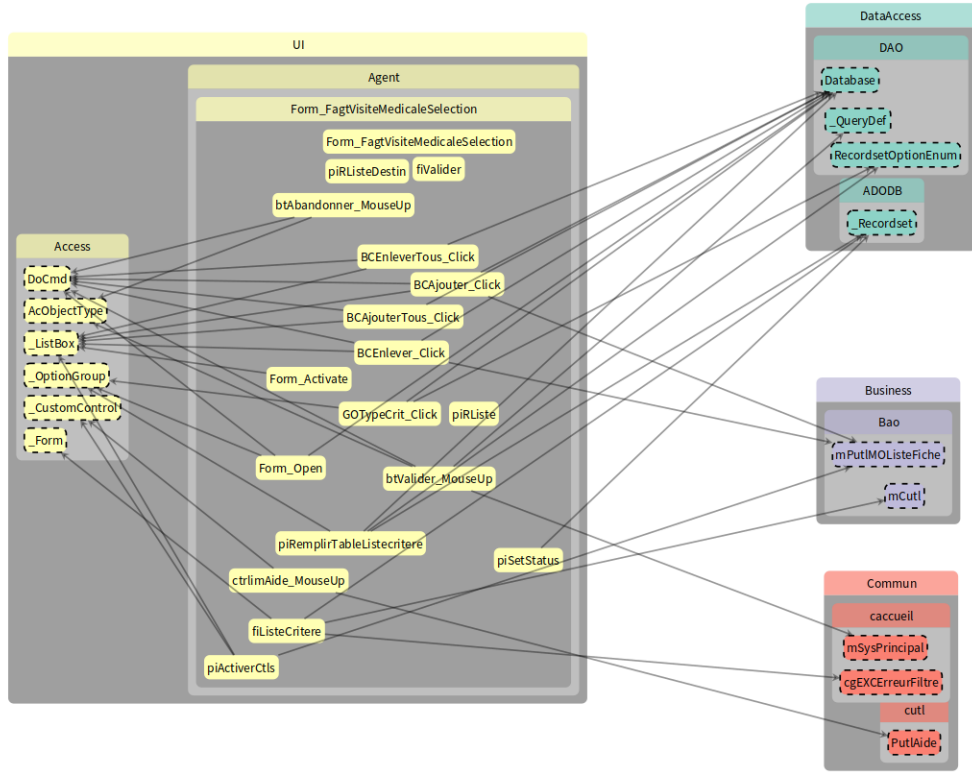
Fig. 10. Architectural dependency graph applied to Form_FagtVisiteMedicaleSelection. We can observe in here a strong dependency on Data Access.
