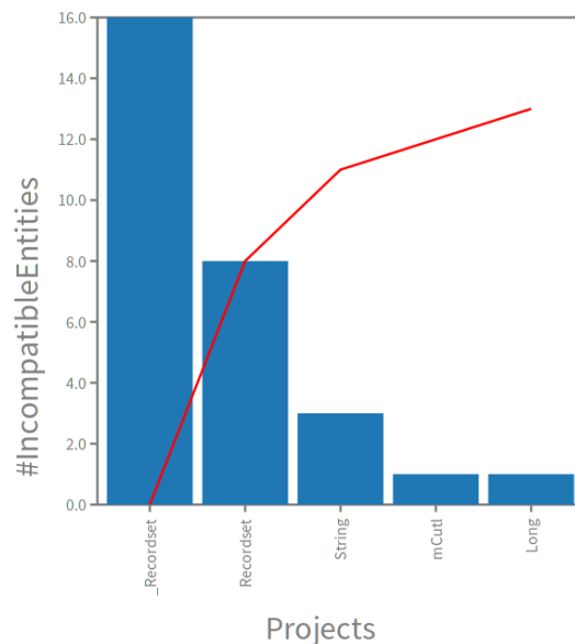
Fig. 11. Analysing fiListeCritere : Dependency complexity metric on Pareto chart.
