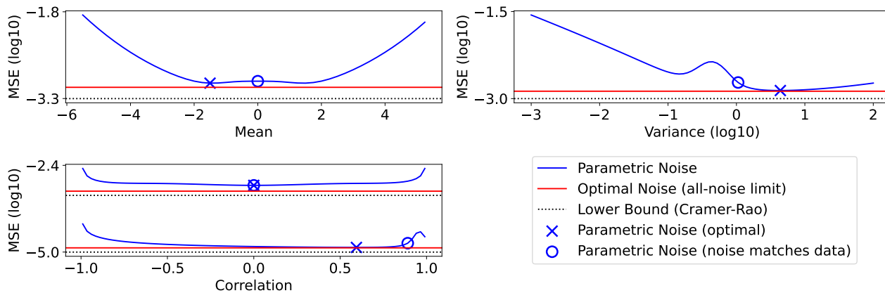
Figure 6: MSE vs. the noise parameter. Top left panel for model (i), Gaussian mean; Top right panel for model (ii), Gaussian variance; Bottom left for model (iii), Gaussian correlation.
