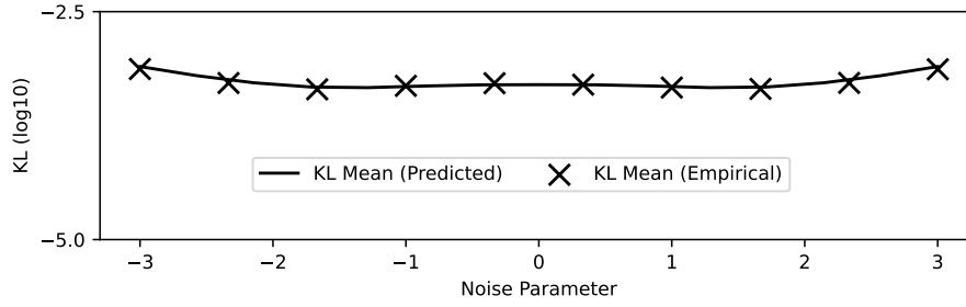
Figure 7: KL vs. the noise parameter (Gaussian Mean). The noise proportion is fixed at 50%.
