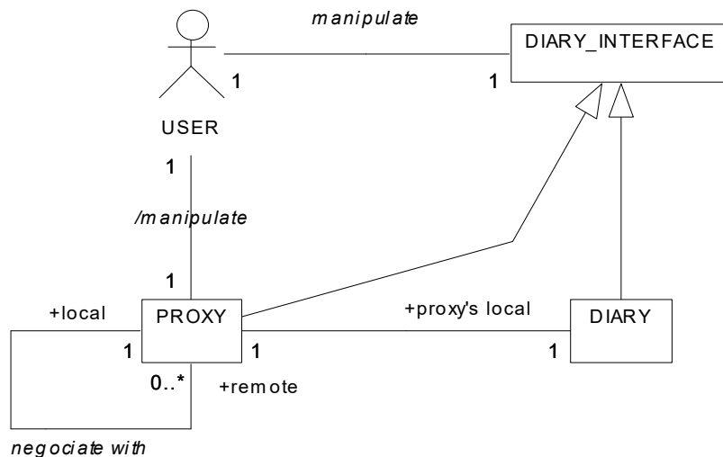
Figure 3: Class diagram of the system before transformation
