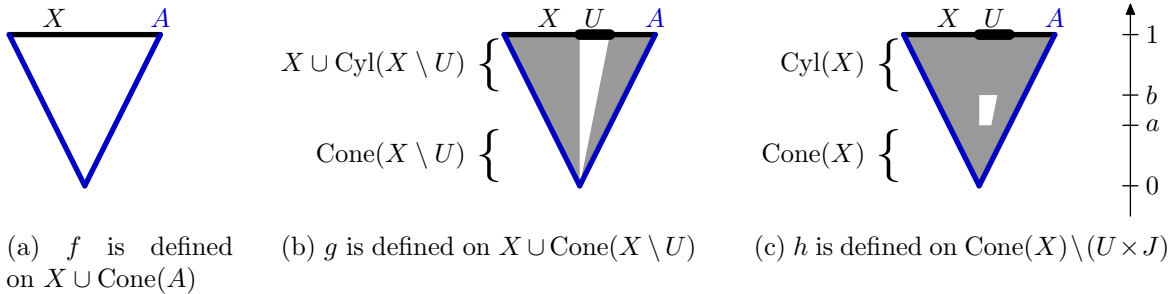
Figure 3: Consecutive extensions of f
