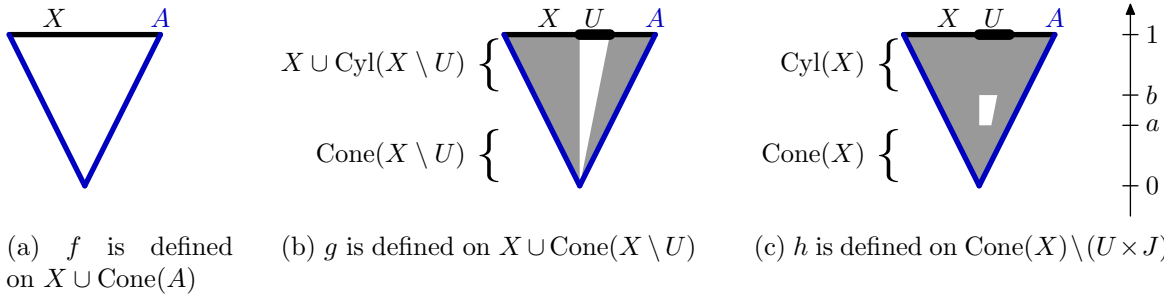
Figure 3: Consecutive extensions of f
