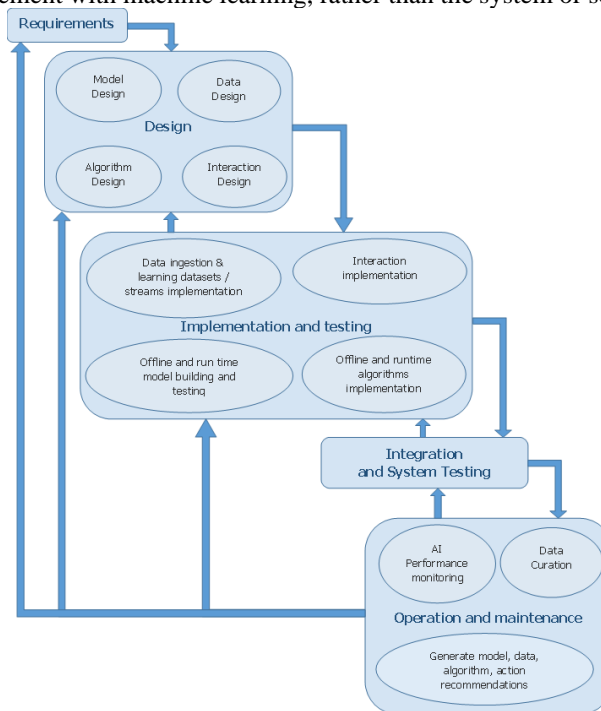
Fig. 1. Machine Learning waterfall diagram outlining human actions
