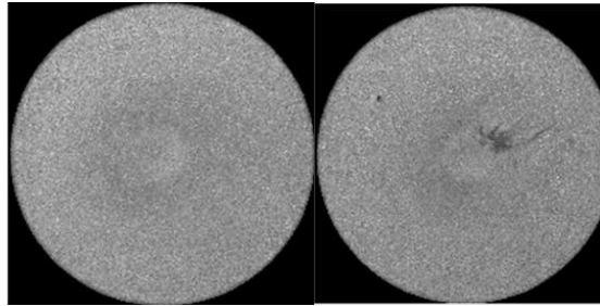
Fig. 3. Vision-based quality inspection showing good (left) and bad (right) quality products Source: courtesy of Philips, through STAR project, ID: 956573, www.star-ai.eu
