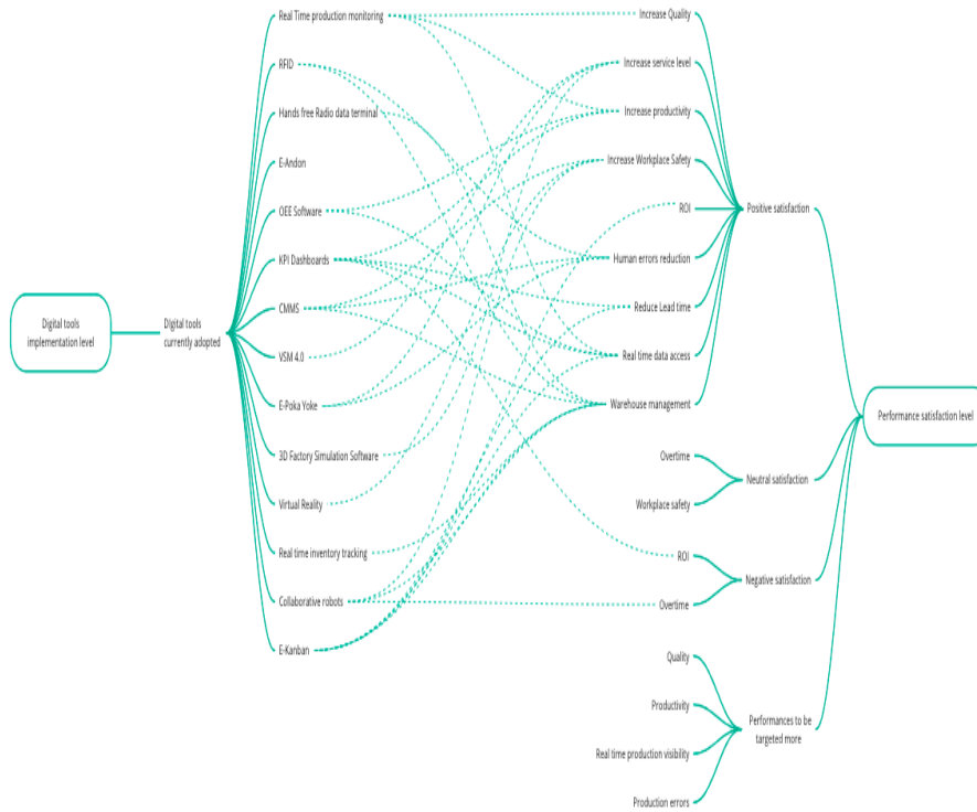
Fig 1. Association Performance-Tool
