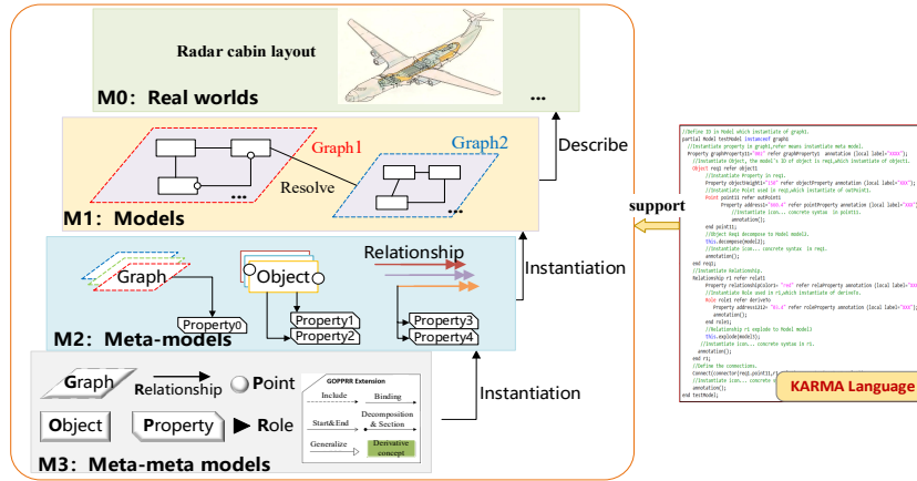
Fig. 2. M0-M3 Domain-specific modeling and GOPPRR
