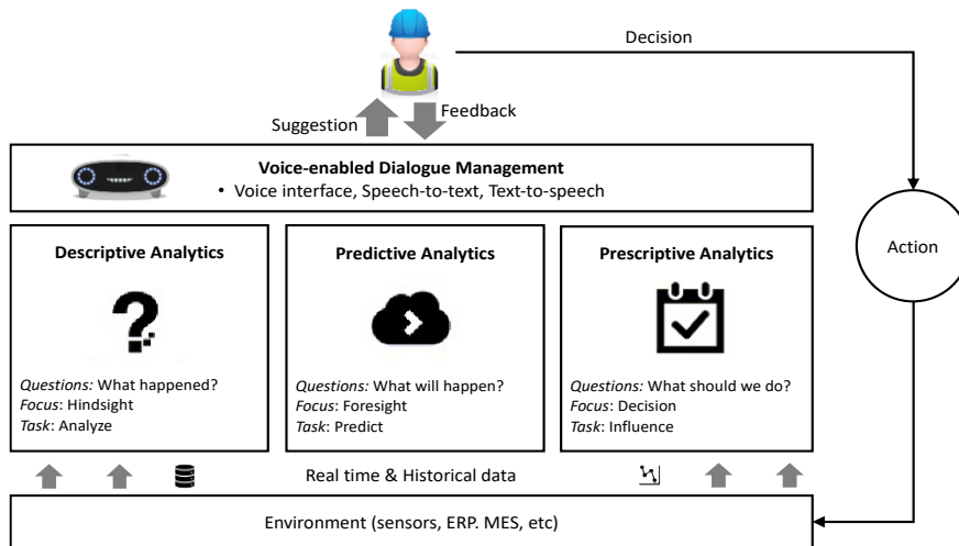
Fig. 1. Augmented Manufacturing Analytics framework
