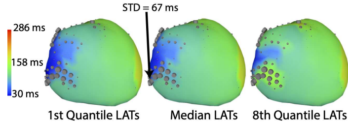
Fig. 4. Spatial distribution of LAT uncertainty illustrated by the median (center) and the minimum (left), and maximum (right) over 8 quantiles. Cylinder sizes represent relative standard deviation of the LAT at each location.
