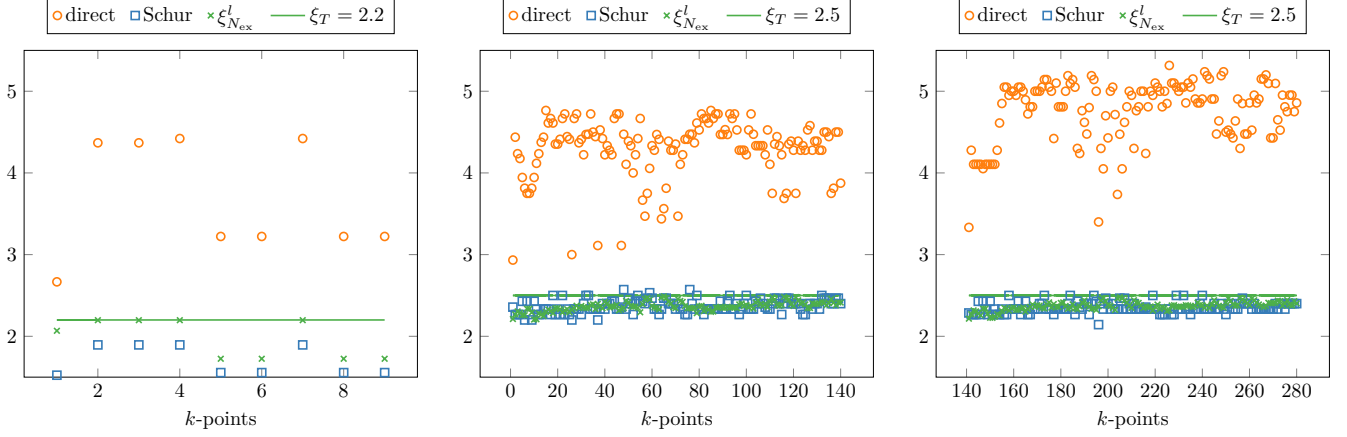
FIGURE 10 – Comparison between the ratio \xi_{N_{ex}}^\ell (x) and the ratios of the measured number of iterations between the first and last occupied bands, with (□) and without (○) the Schur complement (50). On the x -axis is the index of the k -point. [Left] \text{Al}_{40} with 15 additional extra bands. [Left] \text{Fe}_2\text{MnAl} spin \uparrow with 8 additional bands. [Right] \text{Fe}_2\text{MnAl} spin \downarrow with 8 additional bands.
