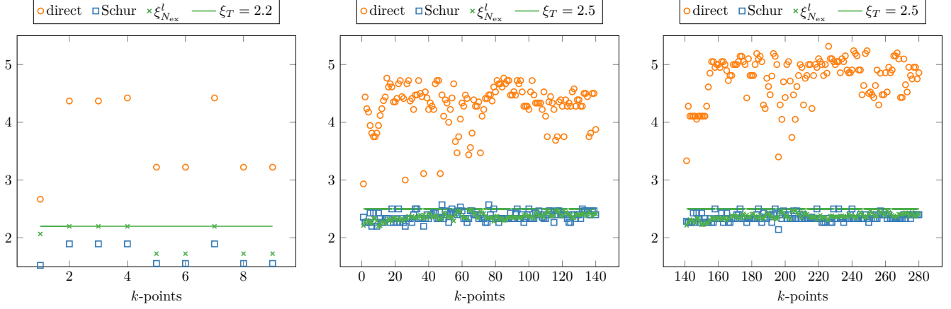
FIGURE 10 – Comparison between the ratio \xi_{N_{\text{ex}}}^{\ell} ( \times ) and the ratios of the measured number of iterations between the first and last occupied bands, with ( \square ) and without ( \circ ) the Schur complement (50). On the x -axis is the index of the k -point. [Left] \text{Al}_{40} with 15 additional extra bands. [Left] \text{Fe}_2\text{MnAl} spin \uparrow with 8 additional bands. [Right] \text{Fe}_2\text{MnAl} spin \downarrow with 8 additional bands.
