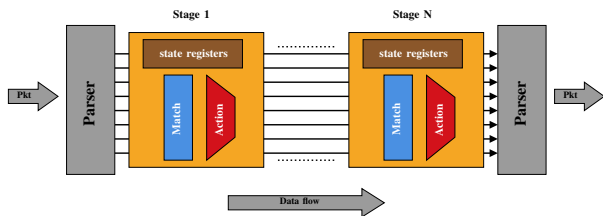
Fig. 1: RMT pipeline: a parser followed by a series of stages. The flow of data is uni-directional
