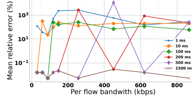
Fig. 10: The mean error when computing various functions for different time-slot values over various bandwidths
