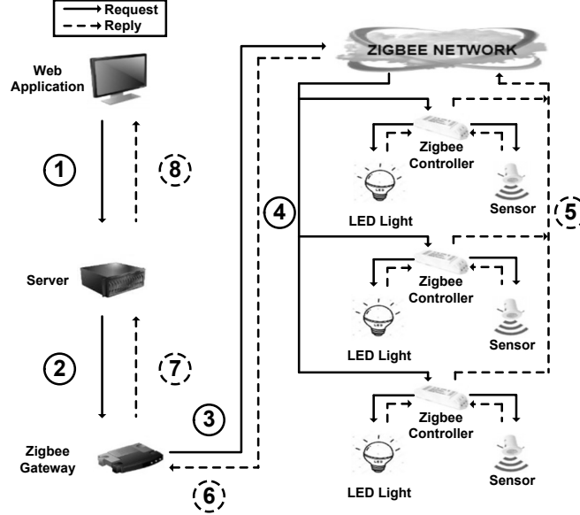
Figure 5. Architecture of Smart Lighting System
