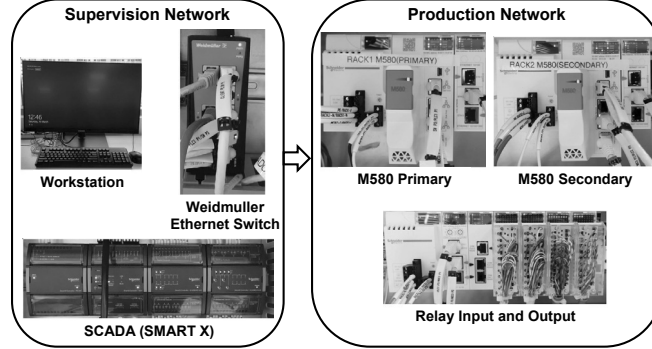
Figure 1. Architecture of the Power monitoring subsystem
