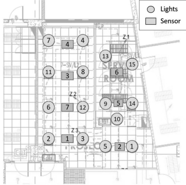
Figure 4. Placement of sensors and lights
