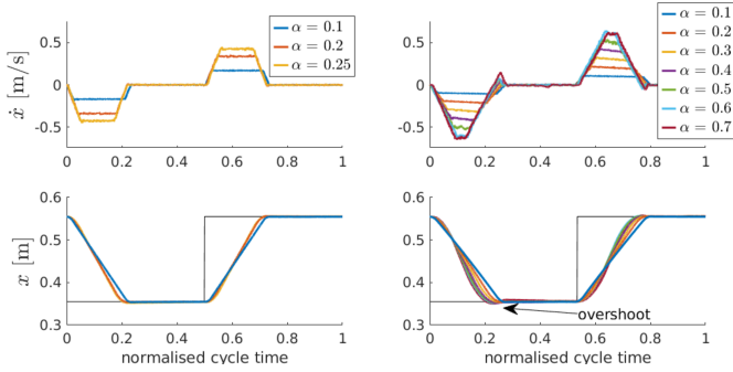
Fig. 6. Recorded evolution of the x -axis position and velocity \dot{x} over the course of one path cycle for different values of capacity scaling factor \alpha . Scaled fixed CS limits approach is shown on the left and the proposed approach on the right. All the plots have been normalised in time of the one cycle.
