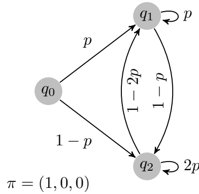
■ Figure 2 Example Parametric Markov chain with parameter p .
