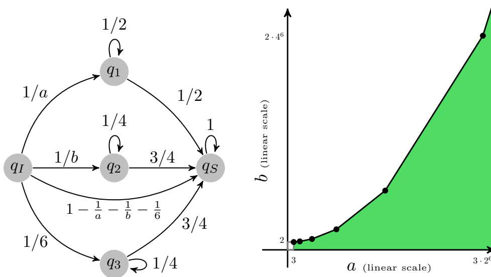
(a) Markov chain with parameters p = (a, b) . (b) Parameters (green) for which \pi \cdot M[p]^n hits T .
