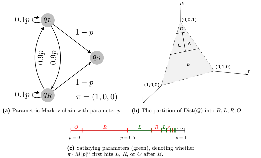
Figure 1 A Markov chain, a partition, and the parameter satisfying the prefix-dependent property B until L .
