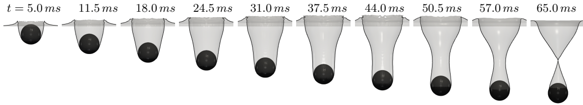
Figure 5. Image sequences showing the water-entry cavity formed by the sphere. Times since the sphere center passed the free surface ( t = 0 ) are shown until the Pinch-Off at t = 65 ms .
