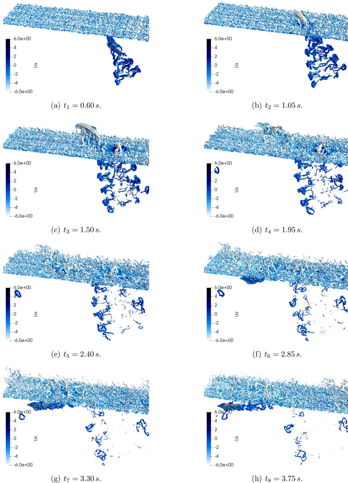
Figure 11. Snapshots of the dolphin with water surface for \theta_0 = 60^\circ and v_0 = 4 m/s. Front view.
