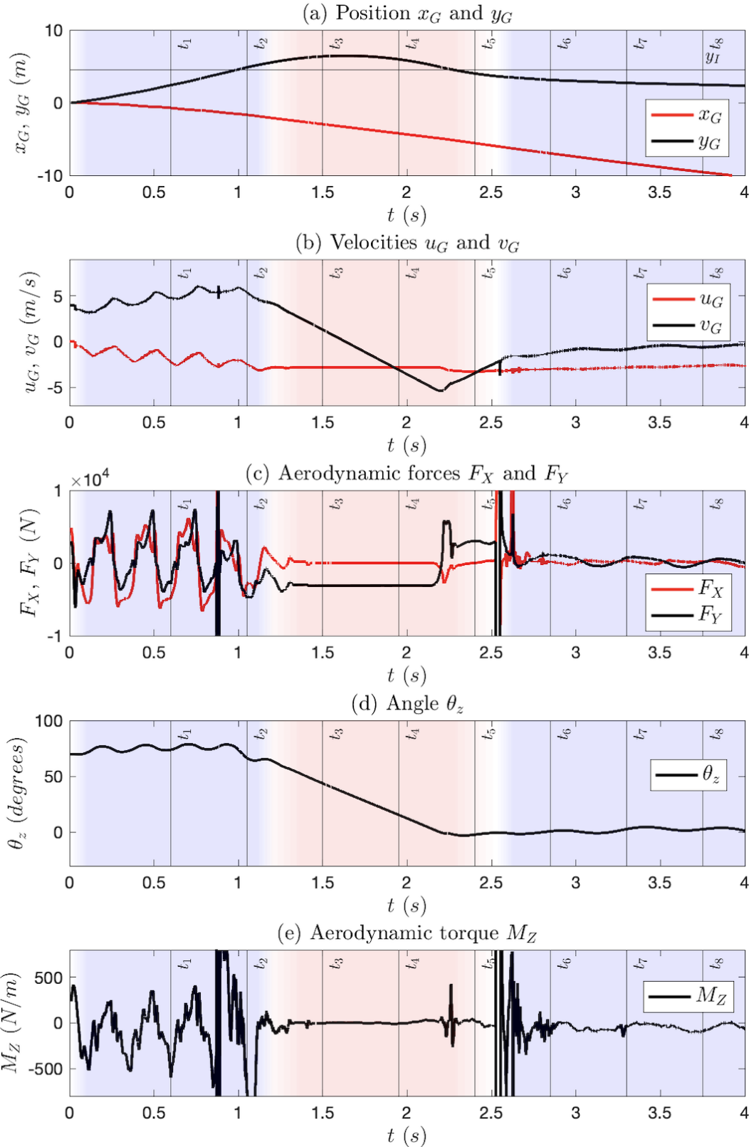
Figure 8. Temporal evolutions of dolphin linear and angular position and velocity, and aerodynamic forces and torques.
