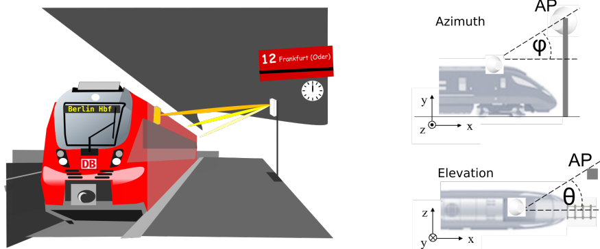
Fig. 4 a) Sketch of the track-to-train communication using mmWave pencil beams b) Azimuth and elevation requirements depending on the angles, COTS hardware used for the trial
