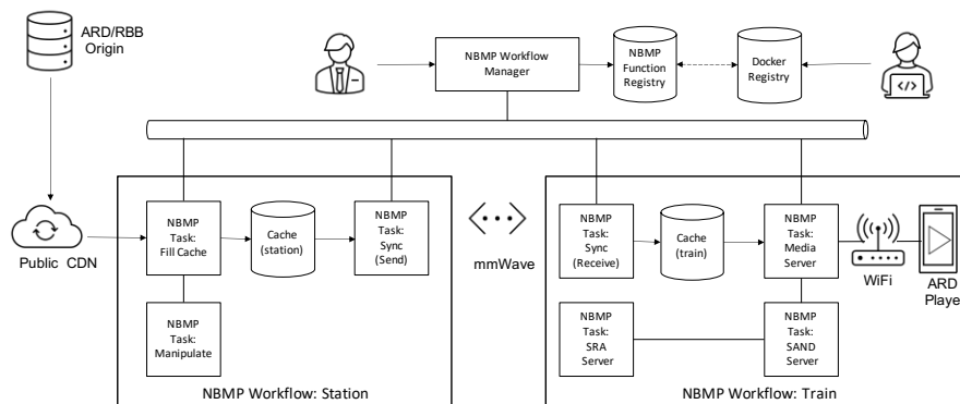
Fig. 3 NBMP Enabled Data Shower Architecture
