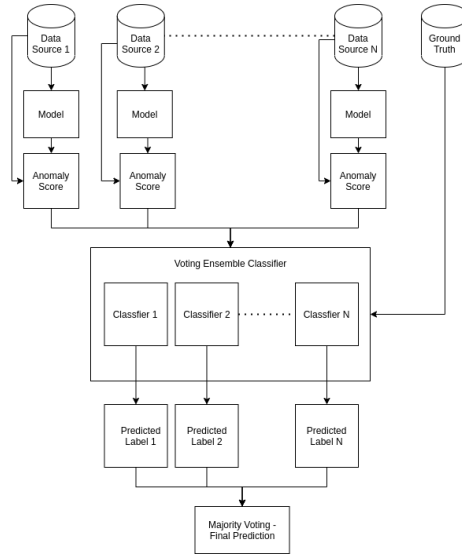
Fig. 2. Architecture of Anomaly Detection Module
