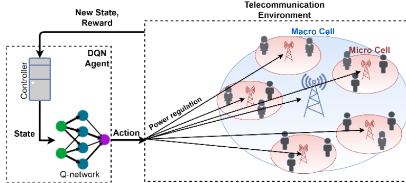
Fig. 1. The interaction cycle between the DQN agent and telecommunication environment.
