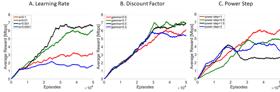
Fig. 2. Accumulated reward for different values of the learning rate \alpha (panel A), discount factor \gamma (panel B) and power step P_S (panel C).
