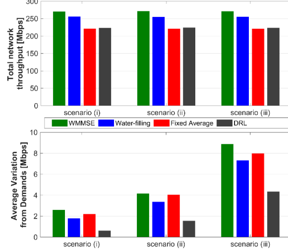
Fig. 3. Comparison amongst methods: DRL performance against Waterfilling , WMMSE and Fixed Average methods for the different validations scenarios in terms of total network throughput (up) and AVD (down) across 1000 network realizations.
