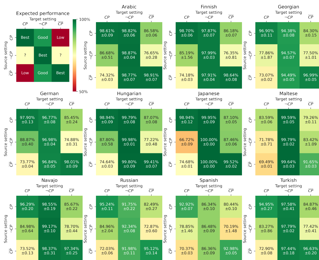
Figure 1: Balanced accuracy of 10 per training setting. In the top left corner, a representation of the expected results
