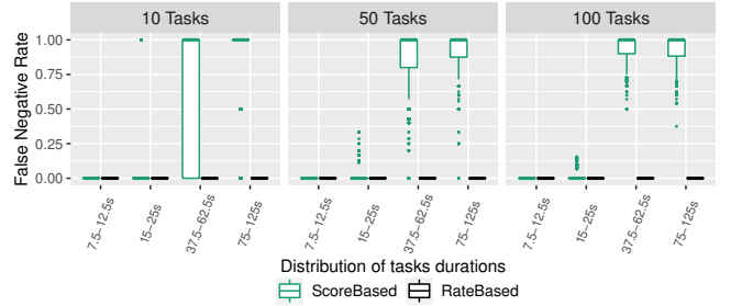
(b) UNIFORMSTARTS-WITHLATENCY
