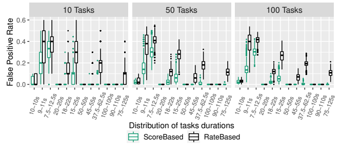
(b) UNIFORMSTARTS-WITHLATENCY
