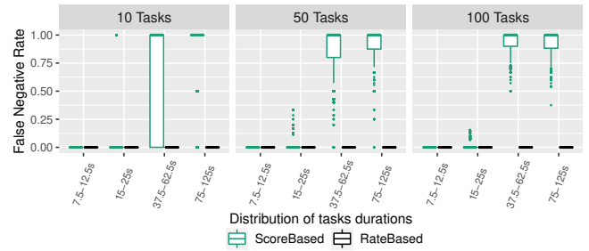
(b) UNIFORMSTARTS-WITHLATENCY
