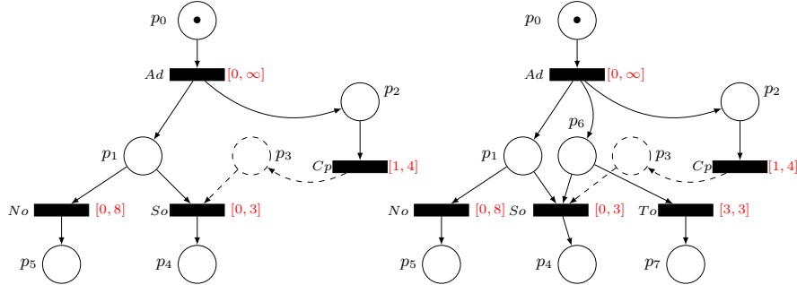
Fig. 2. a) Decoupled time and control in a waiting net. b) ... with a timeout transition.
