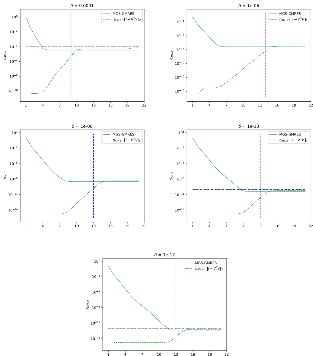
Figure 6: Convergence history of \eta_{AM,b} for the solution of a 3D convection diffusion problem using TT-calculation. The horizontal dashed black line indicates \delta . The vertical dash blue line represents the first iteration where \kappa(V_k) > 4/3 in MGS-GMRES.
