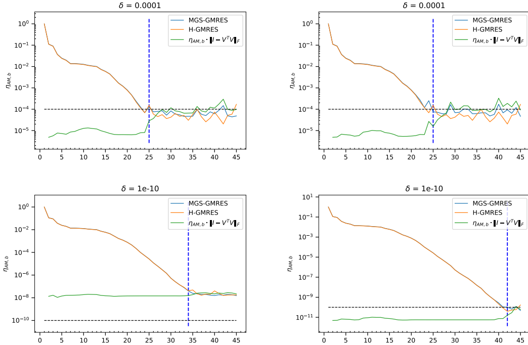
Figure 2: Convergence history of \eta_{AM,b} for gre-343 with ILU(2 \cdot 10^{-1}) using \delta -data componentwise representation with fp32 calculation (left) and fp64 calculation (right). The horizontal dashed black line indicates \delta . The vertical dash blue line represents the first iteration where \kappa(V_k) > 4/3 in MGS-GMRES.
