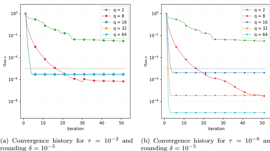
Figure 17: 3-d Poisson problem, comparing preconditioners
