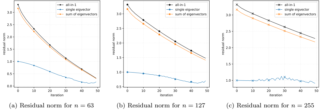
Figure 19: 4-d multiple right-hand side problem, residual comparison
