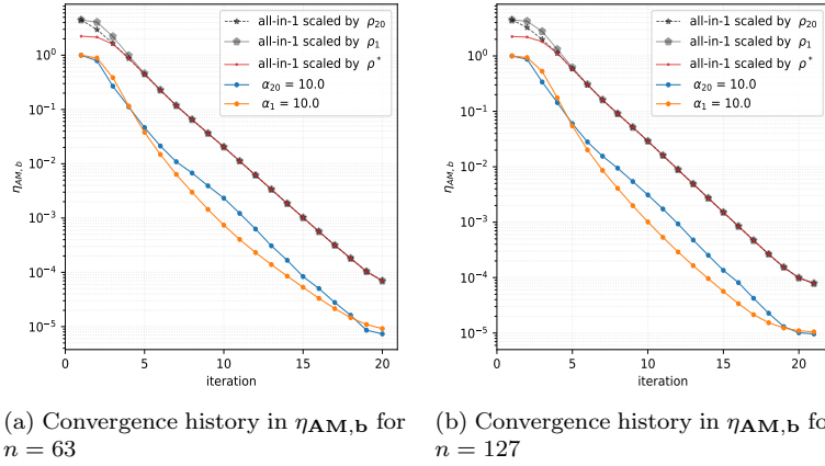
Figure 10: 4-d Heterogeneous convection diffusion \eta_{\mathbf{AM},\mathbf{b}} bound using \delta = \varepsilon = 10^{-5}
