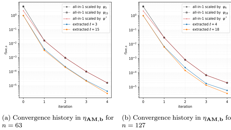
Figure 16: 4-d multiple right-hand side convection-diffusion problem \eta_{\mathbf{AM},\mathbf{b}} bound using \delta = \varepsilon = 10^{-5}
