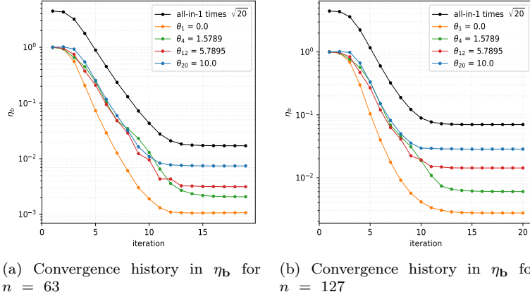
Figure 9: 4-d Heterogeneous convection diffusion \eta_{\mathbf{b}} bound using \delta = \varepsilon = 10^{-5}
