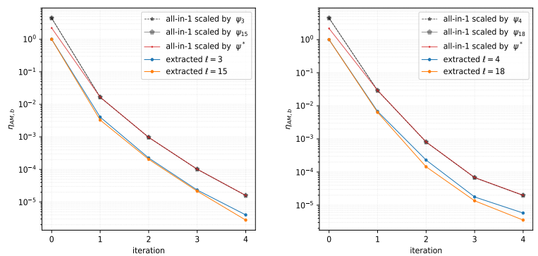
(a) Convergence history in \eta_{AM,b} for n = 63 (b) Convergence history in \eta_{AM,b} for n = 127
