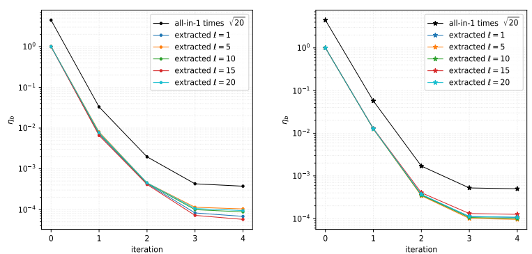
(a) Convergence history in \eta_b for n = 63 (b) Convergence history in \eta_b for n = 127
