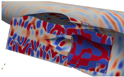
Fig. 15. Industrial test case result: the acoustic pressure is visualized in the flow (at the front) and on the surface of the plane (at the back). The color scale is saturated, so as to see the acoustic pressure on the fuselage, which is much smaller than the pressure in the flow (as one might expect, the noise is much higher inside the engine). The blurry pale part of the flow on the left is the hot part of the jet flow, coming out of the combustion chamber (not represented). It underlines the strong heterogeneity of the flow.
