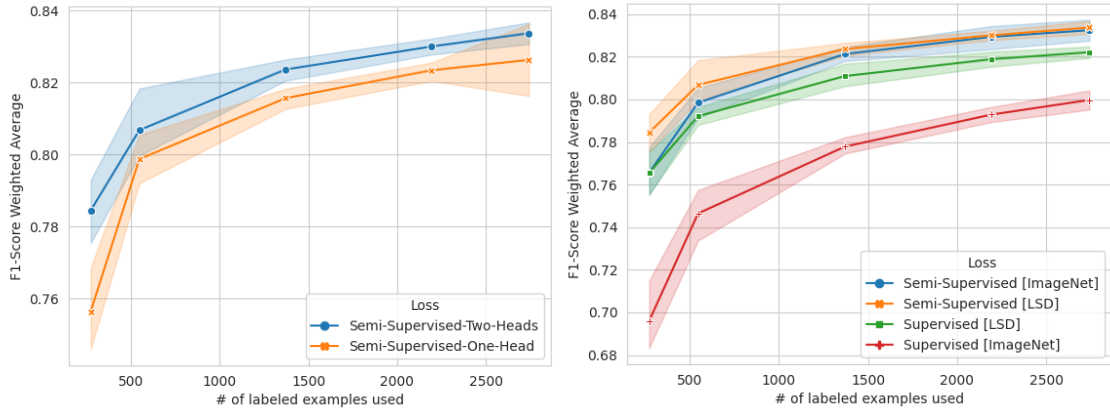
Fig 7 Mean and 95% confidence intervals of F1-score weighted average using all unlabeled images ( n_u = 84967 ) with 10%, 20%, 50% and 100% of labeled images ( n_s = 2742 ). On the left: One-Head vs Two Head semi-supervised learning models presented in Fig. 3. On the right: Semi-Supervised vs Supervised Learning models with different pretraining methods.
