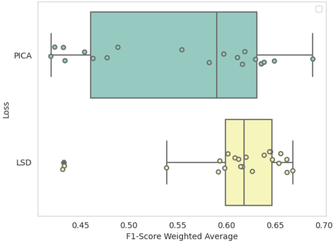
Fig 6 A box-plot showing F1-score weighted average values for each loss using five different values of \lambda over four experiments with different seeds.
