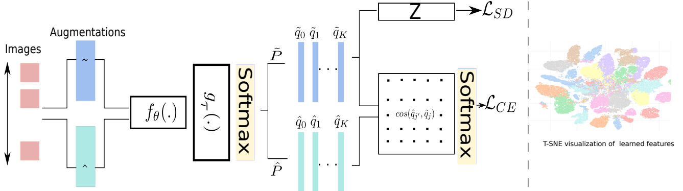
Fig 2 Overview of the deep clustering framework. Two different augmentation schemes ( \tilde{(\cdot)} and \hat{(\cdot)} ) are applied to all input images before passing through the CNN composed of a feature extractor f(\cdot) and a classification head g_\tau(\mathbf{x}) = p = \{p_1, \dots, p_K\} . This framework can serve as an unsupervised classification model when no labeled examples are available. \mathbf{P} is the cluster prediction matrix of all images in \mathbf{U} and \mathbf{Z} is the cluster size distribution. A T-SNE visualization of the learned features and their assigned clusters represented by different colors is shown on the right.
