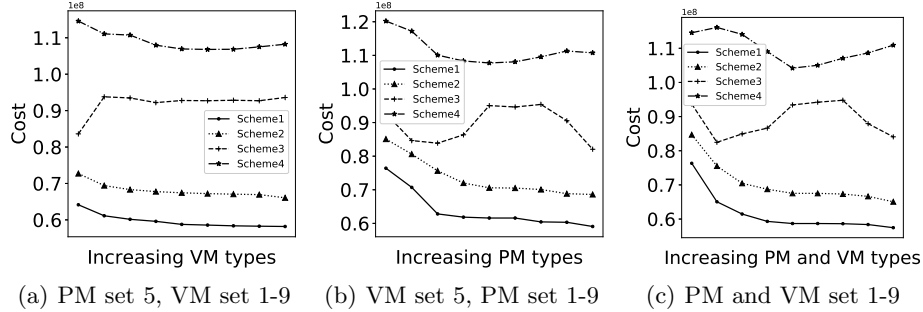
Fig. 3. Four compared schemes' adaptability on different distribution of datasets
