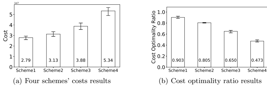
Fig. 2. Four compared schemes' cost results to solve the JVMSP problem
