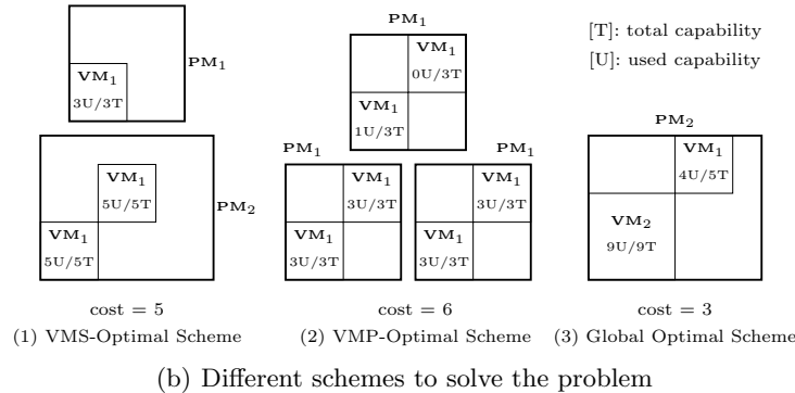
Fig. 1. VM selection and placement in clouds
