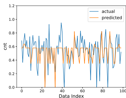
(b) Predicted result from decision tree model.
