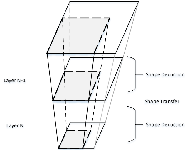
Fig. 2. An example for layer fusion process
