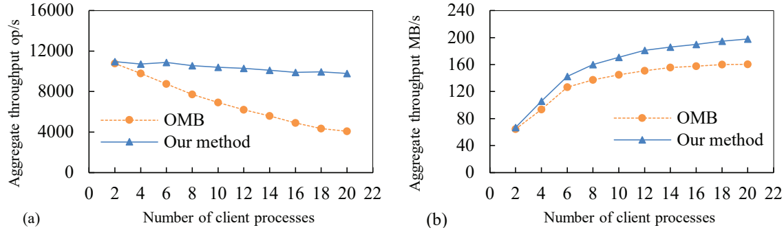
Fig. 3. The aggregate throughput: (a) metadata; (b) small files.
