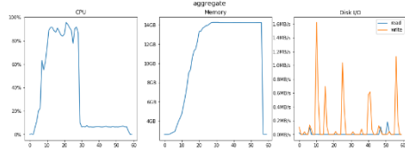
Fig. 5. aggregate resource consumption
