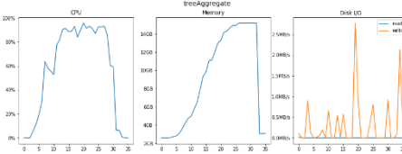
Fig. 6. treeAggregate resource consumption
