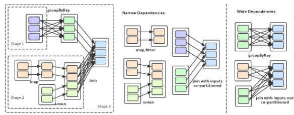
Fig. 2. Wide vs Narrow Dependencies
