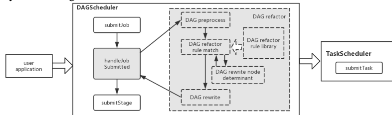
Fig. 3. System architecture diagram
