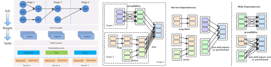
Fig. 1. The architecture of Spark.
