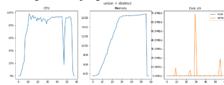
Fig. 7. union + distinct resource consumption
