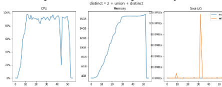
Fig. 8. distinct + union + distinct resource consumption
