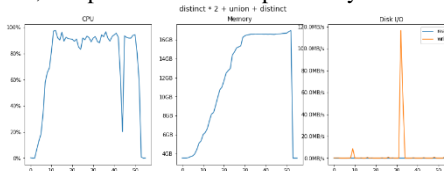
Fig. 8. distinct + union + distinct resource consumption
