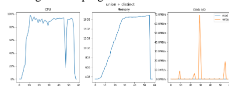
Fig. 7. union + distinct resource consumption
