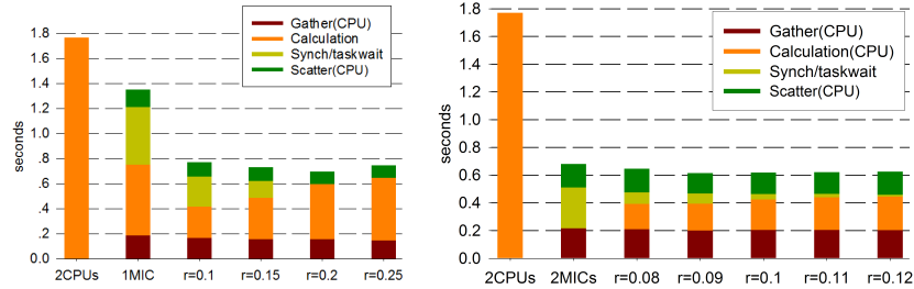
Fig. 2. Performance of CPU+1MIC (left) and 2MICs (right) with problem size 256 \times 256 .
