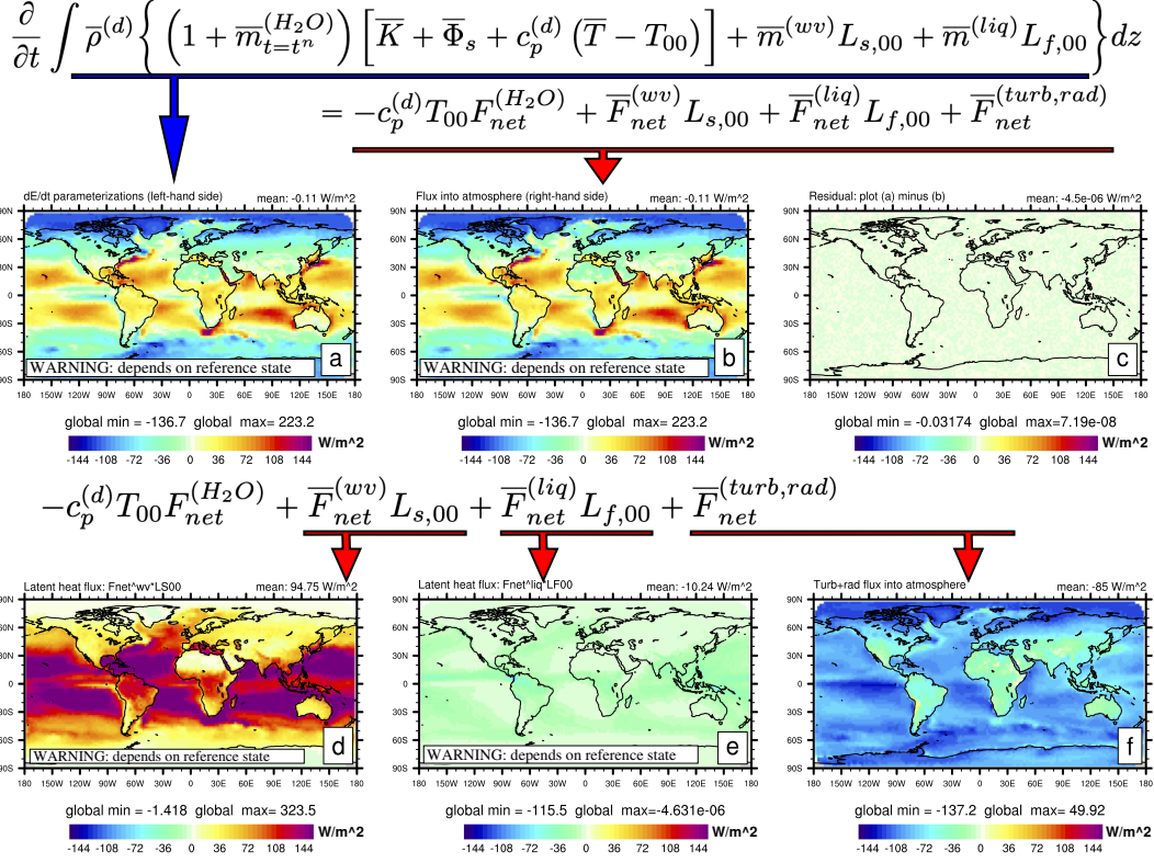
Figure 2. One year average of vertically integrated terms in the CAM parameterization energy budget equation based on an Atmospheric Model Intercomparison Project (AMIP)-like simulation cycling over year 2000 SST's. (a) Left-hand side of (111), (b) right-hand side of (111), (c) residual, (d-e) latent heat flux terms, (111), (f) turbulent/sensible and radiative flux F^{(turb,rad)} . Note that plots (a), (b), (d), and (e) depend on the specific reference state used in CAM (ice enthalpy reference state with T_{00} = 0^{\circ}C ) whereas (c) does not. In the upper right corner of each plot is the global average of the term in question.
