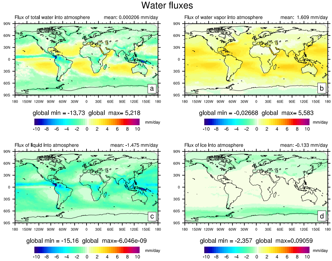
Figure 5. One year average surface fluxes of water (fluxes are positive for inflow into the atmosphere; units are mm/day ; in SI units the flux is kg/m^2/s which is converted to mm/day by using that 1cm^3 of water is 1gm and that the length of day is 86400s ). (a) is total net water flux and (b,c,d) is the breakdown into net water vapor, liquid and ice flux, respectively. Note the similarities, in terms of pattern, between the total water flux and the dry-mass adjustment in Figures 3d and 4b which accounts for the total energy imbalances associated with water leaving/entering the column.
