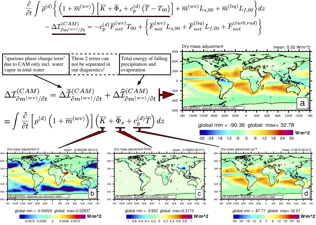
Figure 3. (a) One year average of the total energy budget imbalance in each physics column, \Delta \mathcal{I}_{\partial m^{(wv)}/\partial t}^{(CAM)} [W/m 2 ], associated with updating total water (which in CAM is only water vapor); see also (113). The global average of \Delta \mathcal{I}_{\partial m^{(wv)}/\partial t}^{(CAM)} is shown in the upper right corner of each plot. The imbalance can be split into a “spurious phase change” term (115) and a term (116) associated with falling precipitation and evaporation. These two terms are, unfortunately, not separable in our diagnostics (the former is, however, likely small). (b,c,d) show the break-down of the kinetic, geopotential and enthalpy terms, respectively. Observe that the enthalpy term is two and three orders of magnitude larger than then kinetic and geopotential energy parts, respectively.
