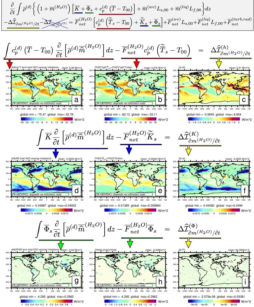
Figure 7. A breakdown of the imbalance term in W/m^2 (shown in Figure 6) associated with (row 1) enthalpy, (row 2) kinetic and (row 3) geopotential energy, respectively. Note that plot (i) should be exactly zero, however, due to truncation errors in computing the diagnostics (and mass clipping - see section 4.4) it is not round-off.
